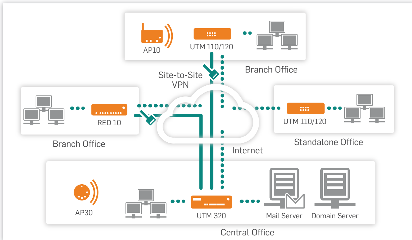
Deployment scenario of Sophos UTM 320
